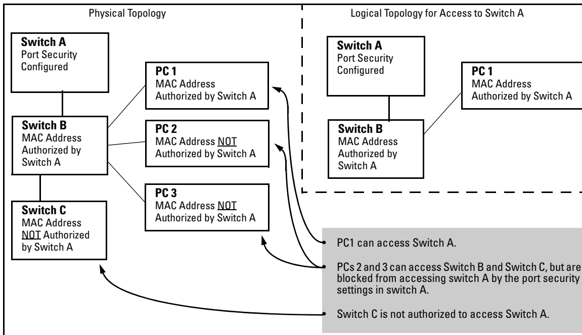
Figure 13-1. Example of How Port Security Controls Access
